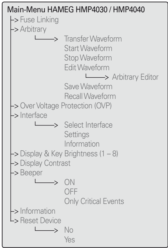
Fig. 5.2: Menu principal HMP4030/4040
